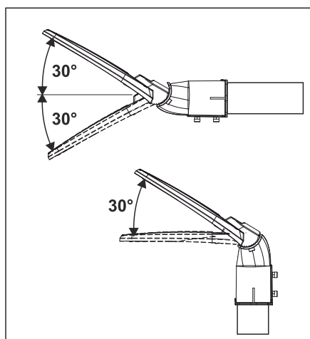
Technical drawing
