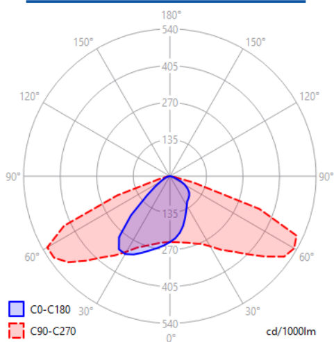
Photometric solid
